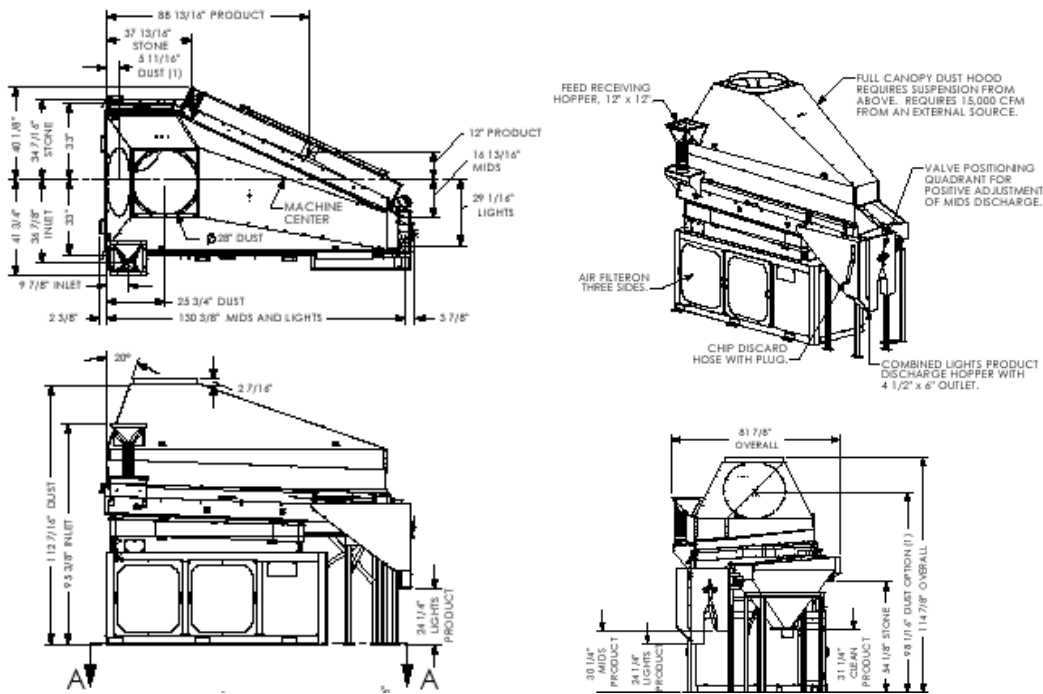
Shown with Optional Full Hood and split middling hopper, but less return conveyor
